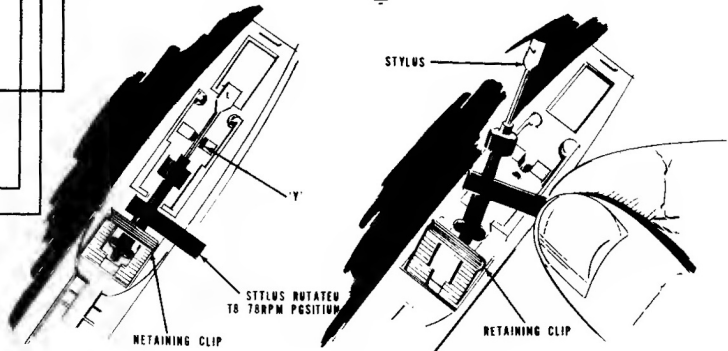
STYLUS REPLACEMENT
